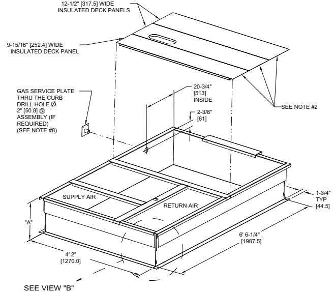
CERTIFIED DRAWING
